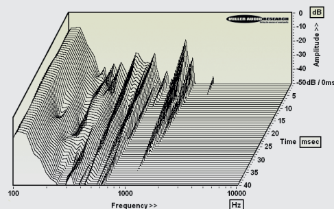
ABOVE: Cumulative resonant decay spectrum, illustrating various bearing housing, pillar and arm vibration modes spanning 100Hz-10kHz over 40msec
